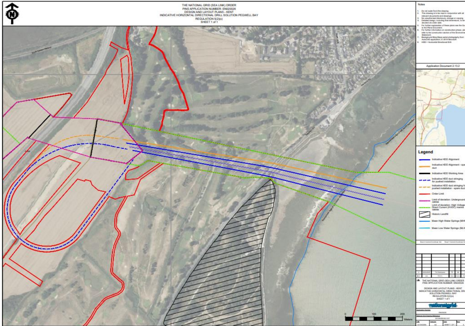
Figure 1.1 Application Document 2.13.2 Design and Layout Plans – Kent Indicative Horizontal Direction Drill Solution Pegwell Bay.
